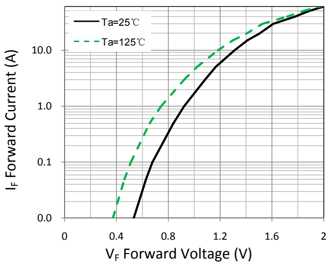
Figure 1. Forward Characteristic(typ.)
